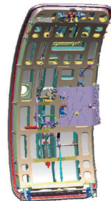
Passenger door with support arm
